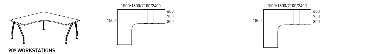
90° WORKSTATIONS
