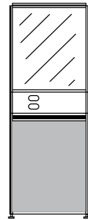
Solid panel to 800mm (approx.) with power duct and glazed panel above (single or double 6mm glass) Optional excess cable pockets shown
