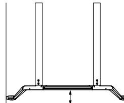
Splayed leg 150mm overhang
